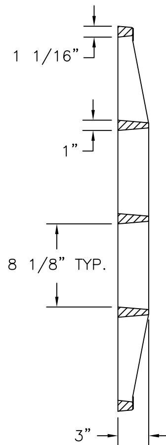
GRATE SECTION
