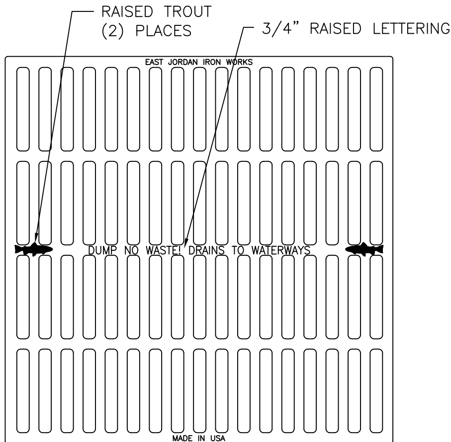
GRATE TOP VIEW
