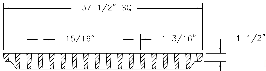
GRATE SECTION
